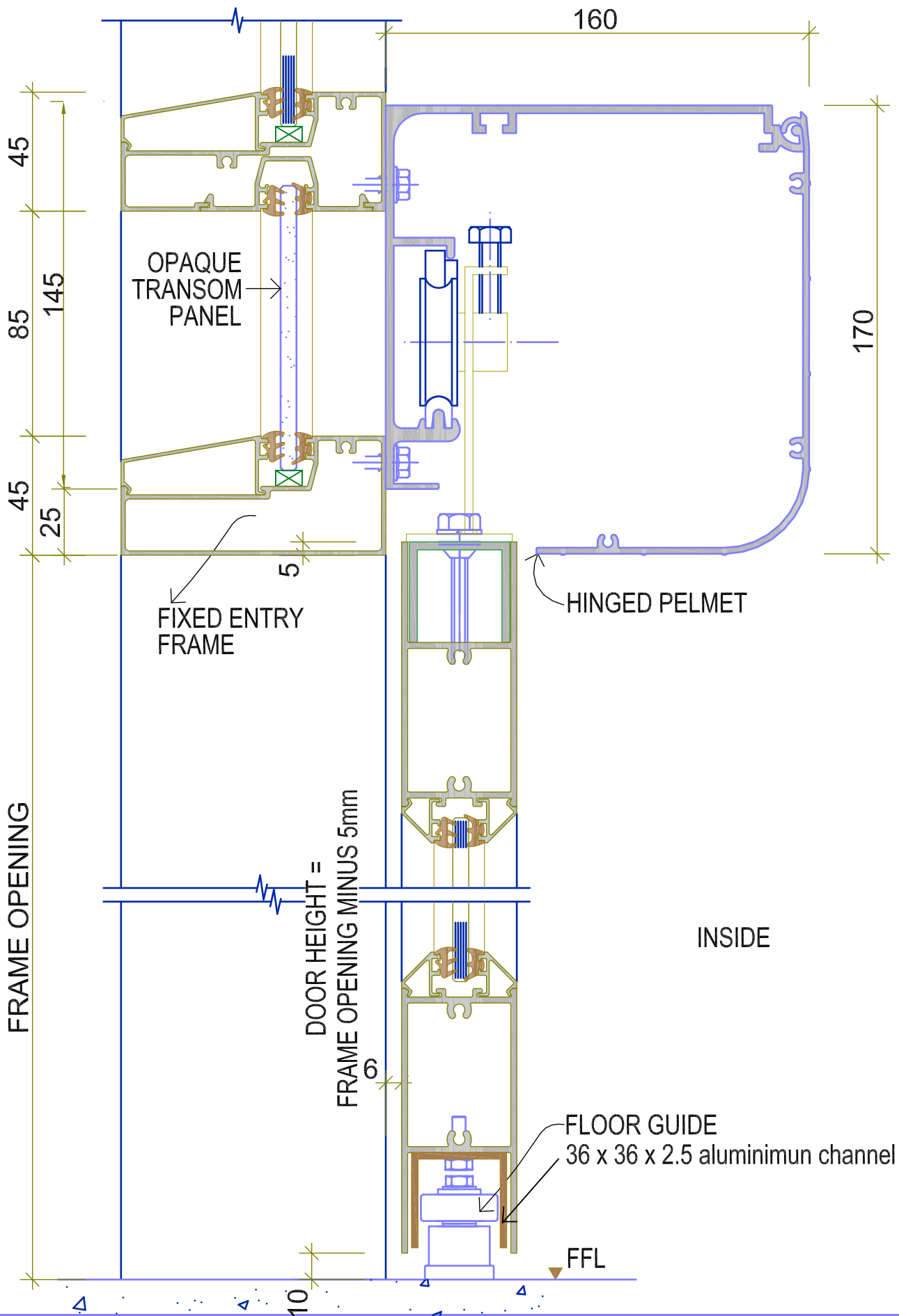
HALF FULL SIZE VERTICAL SECTION THROUGH ULTRASLIDE SD AUTOMATIC DOOR OPERATOR. TRANSM MOUNTED TO ALUMINIUM FRAMING WITH ALUMINIUM DOOR LEAVES
